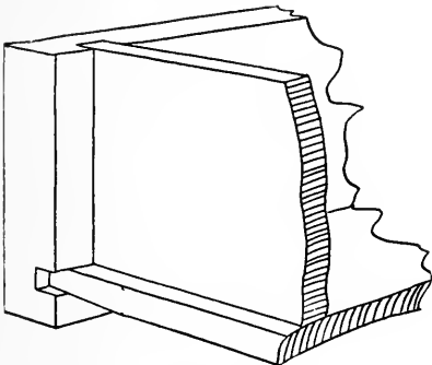
FIG. 436. CONSTRUCTION OF BACK.
